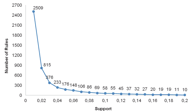
Fig. 3. Amount of rules found x used support figures
