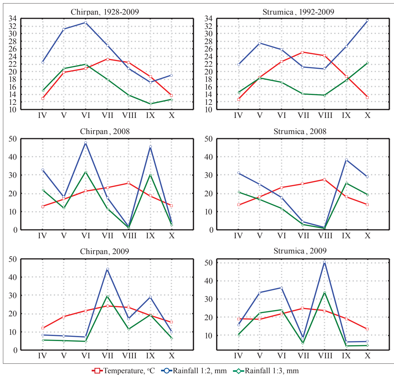
Fig. 1. Drought periods in Chirpan (Bulgaria) and Strumica (Macedonia)
