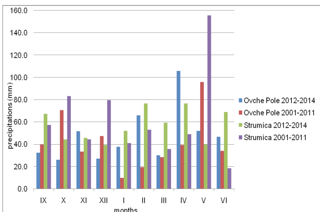
Fig. 2. Monthly sum of precipitations (mm) for period of study and long-term period in Ovche Pole and Strumica locations
