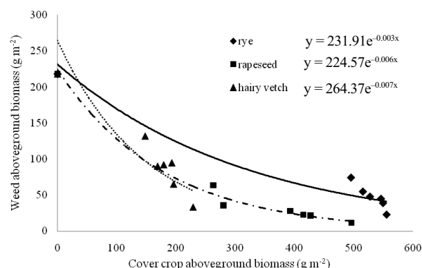
Fig. 3. Exponential decay model describing the relationships between the cover crop aboveground biomass and the total weed aboveground biomass measured at cover crop suppression. Equation for the model is y = ae^{-kx}
