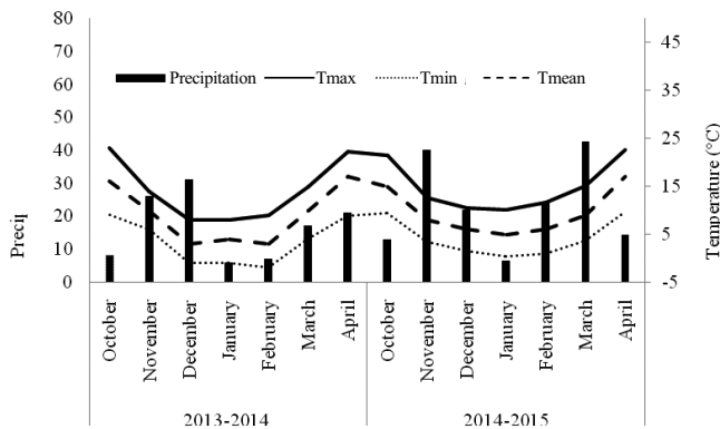
Fig. 1. Climatic data along the growth period of cover crops: (left) the first (2013–2014) and (right) the second (2014–2015) season of cover crop studies from a climatic station situated at the experimental site
