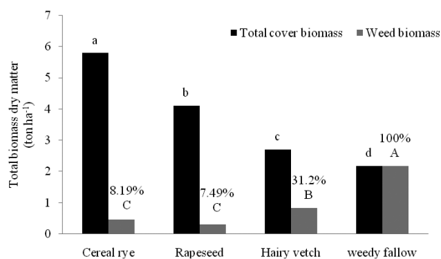
Fig. 2. Total cover biomass at cover crop incorporation (cover species + weeds) and weed percent at total cover biomass. Means without common letters are significantly different according to LSD (0.05) among biomass dry matter (total biomass or weed percent)
