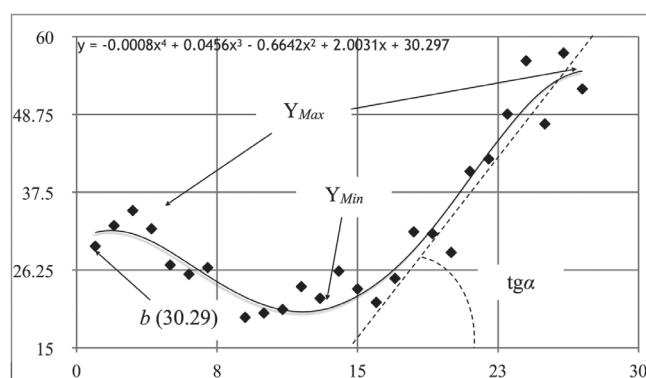
Fig. 1. The typical grain and grain legumes yields dynamics during 1991-2017 and the approximation of the trend by fourth degree polynomial
