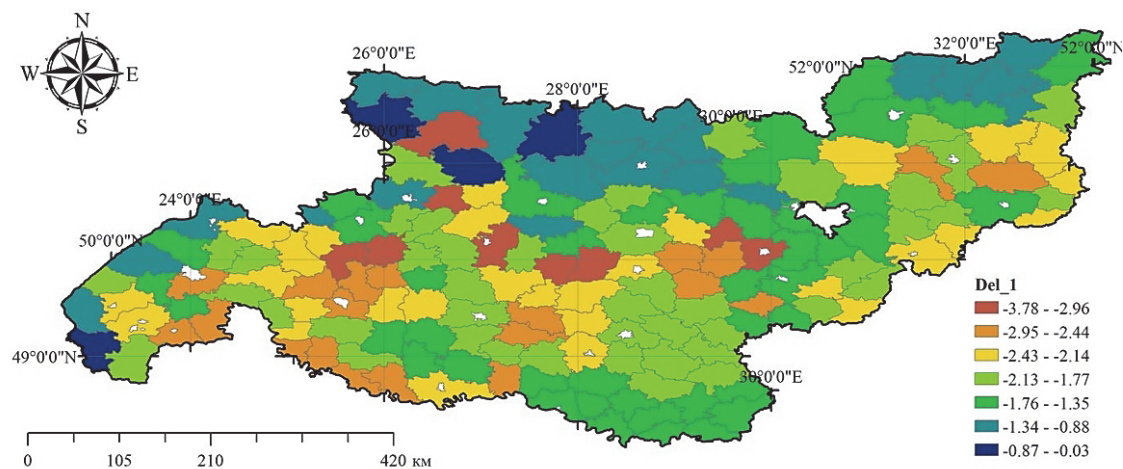
Fig. 4. Spatial variation of the maximum rate of yields decline
