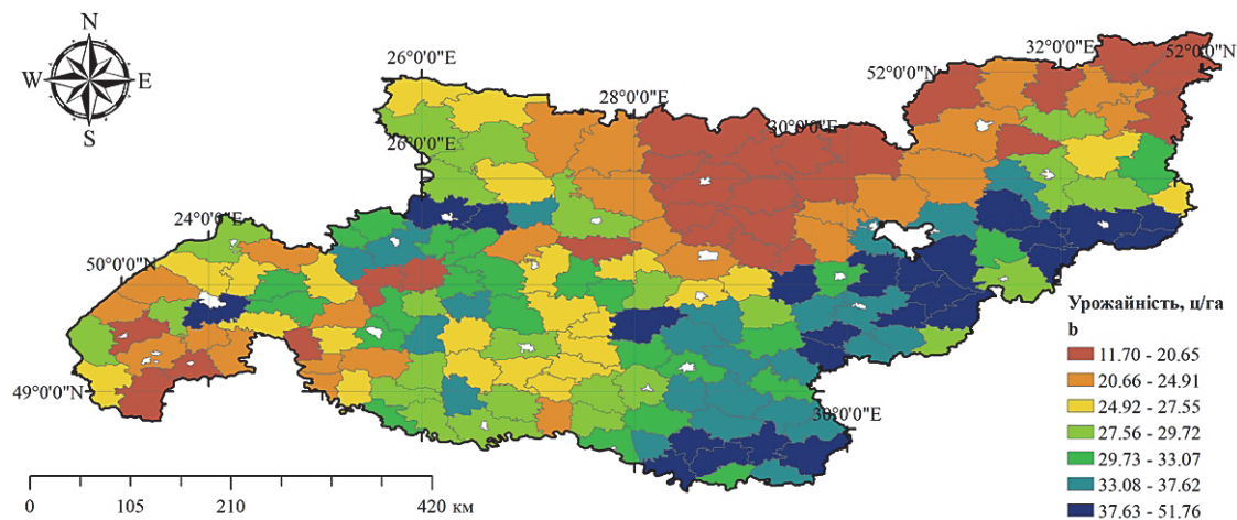
Fig. 3. Spatial variations in the level of crop yields in the initial period of research (constant b of the regression equation)
