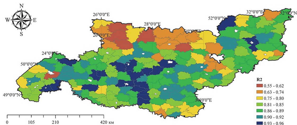
Fig. 2. Spatial variation of the coefficient of determination of the regression model
