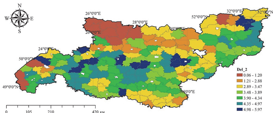
Fig. 5. Spatial variations of the maximum rate of yields increase
